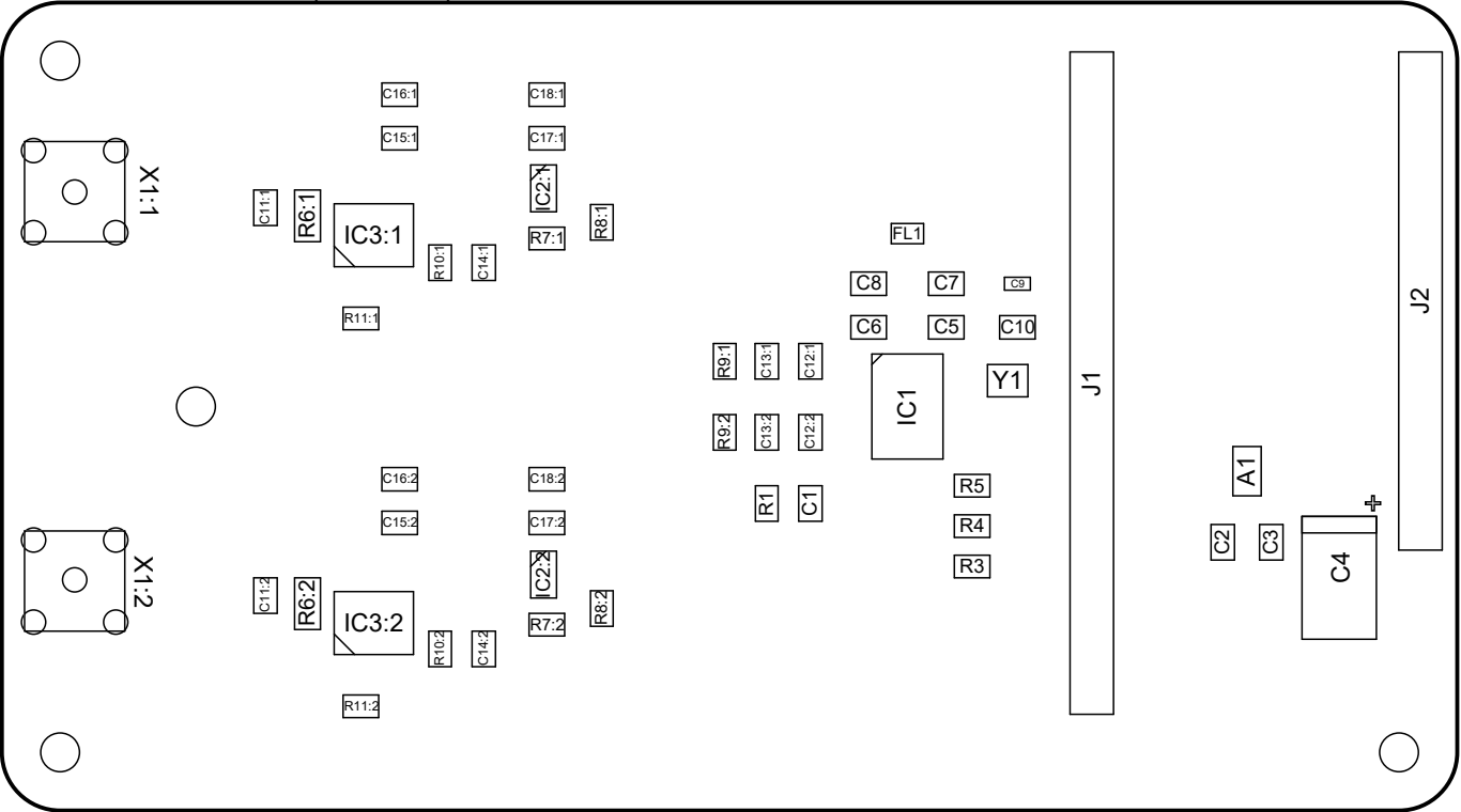
View from Bottom side (Scale 2:1)
