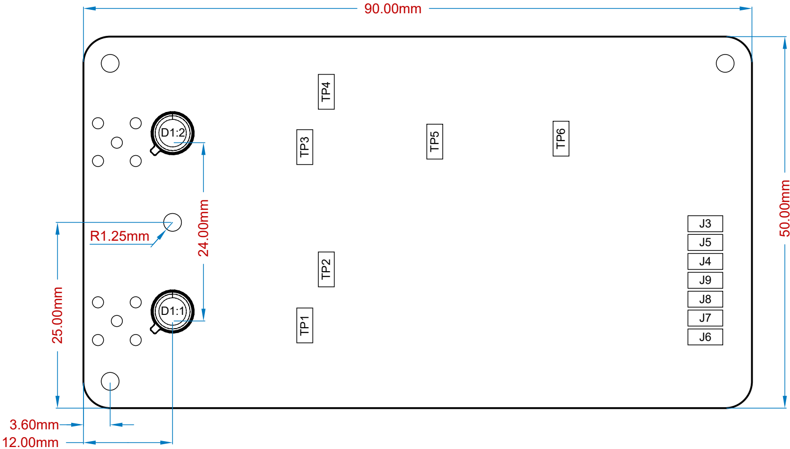
View from Top side (Scale 2:1)
